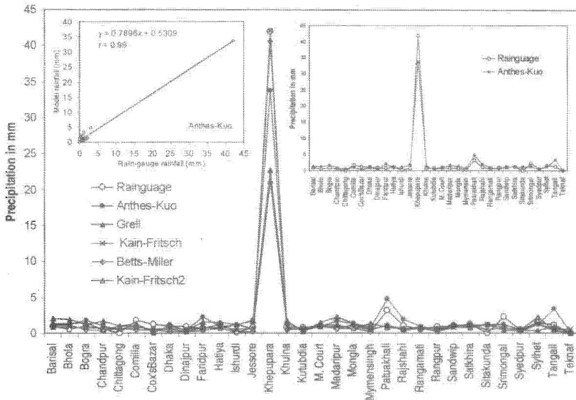
Fig. 5. Comparison of MM5-outputs with rain-gauge data at different locations throughout Bangladesh (inset shows the best trend of Anthes-Kuo and its correlation with rain-gauge) from 31 March to 05 April 2002
