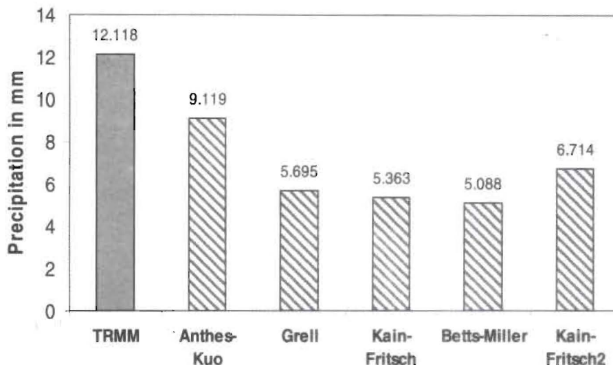
Fig. 3. Comparison of simulated precipitation in BD area for 5 cumulus options of MM5 with that of TRMM value for 138 hrs of simulation
