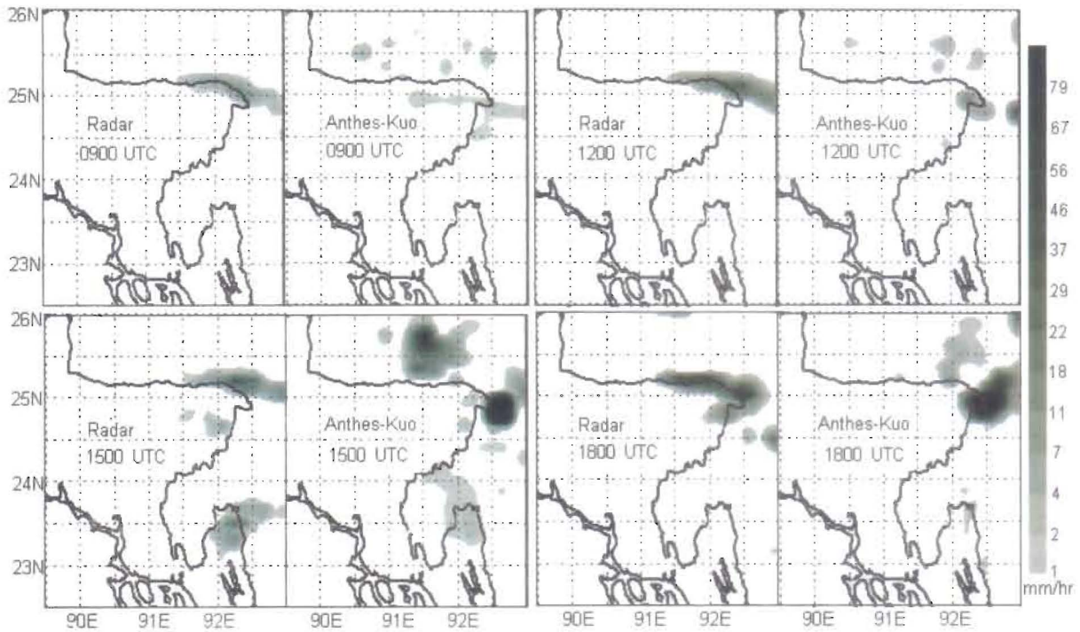
Fig. 6. Display of precipitation for Radar and Anthes-Kuo option at different time of 20 May 2002
