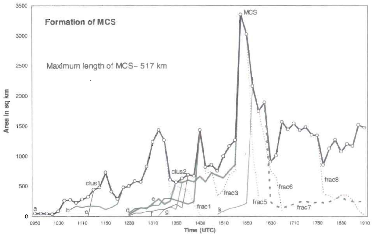
Fig. 7. Area of individual cells, clusters and MCS. Area of the cells h, i, j and fraction frac2, frac4 are not shown because their life time were very short
