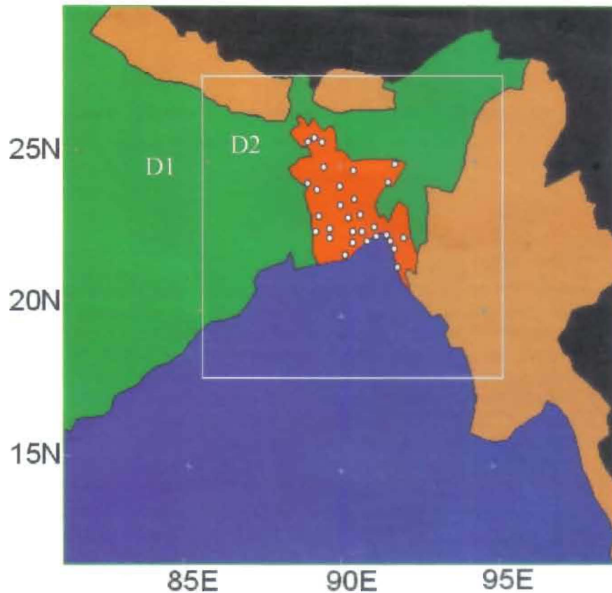
Fig. 1. Analyzing domain to run MM5 (dots indicate the rain-gauge locations)
