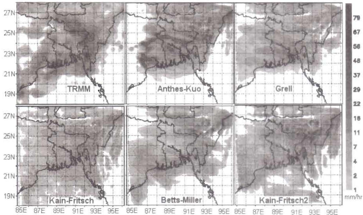
Fig. 2. Structural display of average precipitation in D2 for TRMM 3B42RT and MM5 options from 31 March to 05 April 2002.
