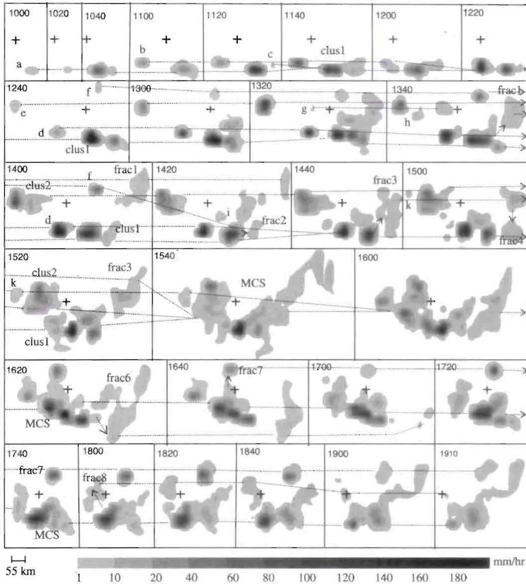
Fig. 8. Structures of cells, clusters and MCS with time (in UTC) and location. Plus mark indicates the position 92.5° E and 25.5° N taken as the relative reference point
