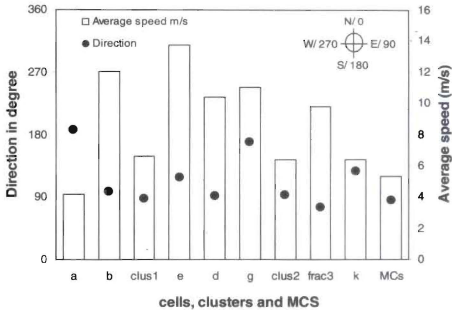
Fig. 9. Speed and direction of cell, cluster and MCS.
