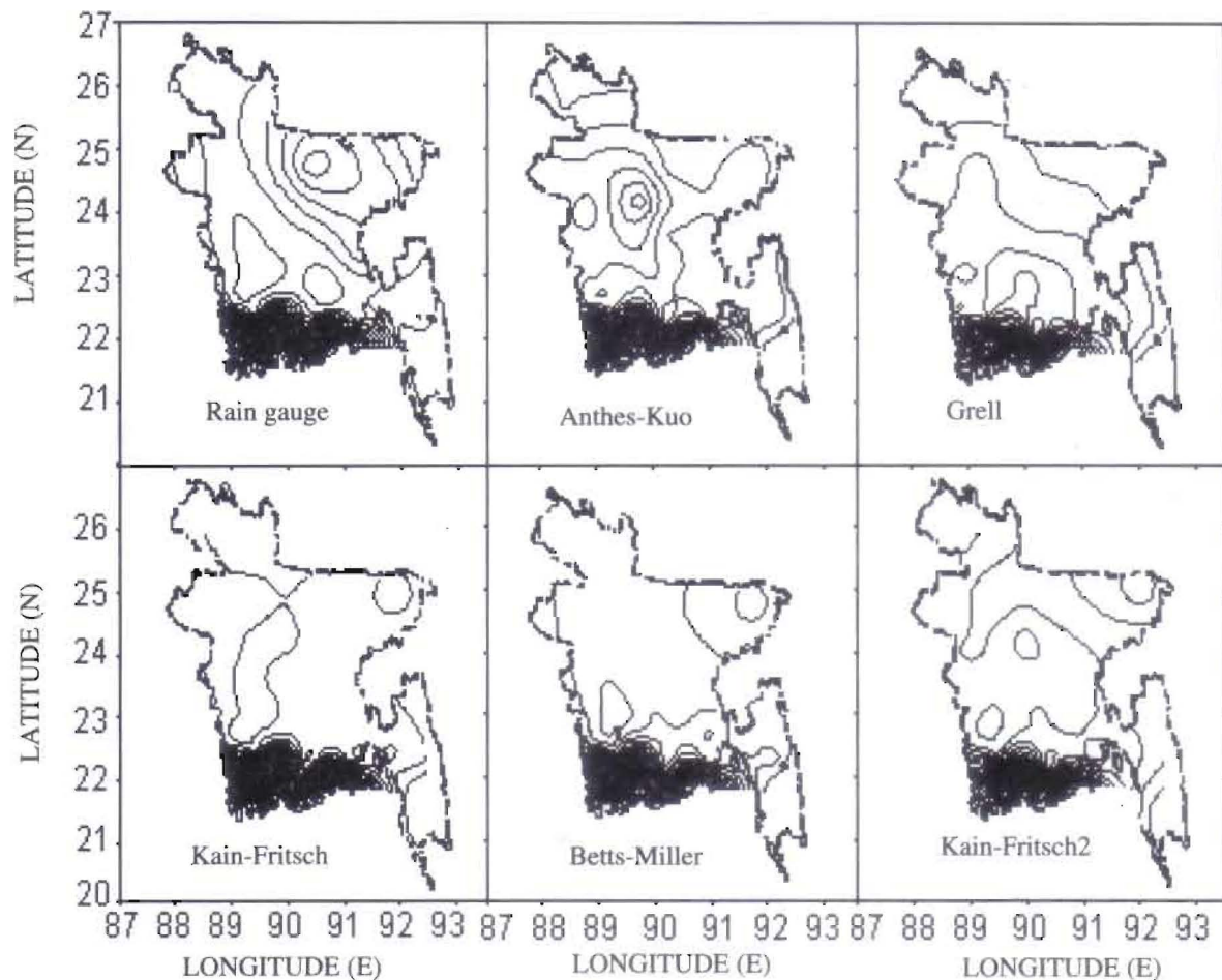
Fig. 4. Comparison of rain gauge data with precipitation simulated by five cumulus MM5 options from 31 March to 05 April 2002
